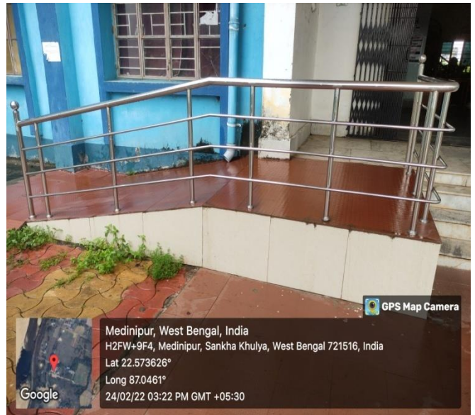
Wheel Chair Access Ramp
